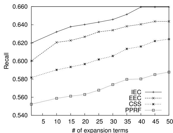
Figure 3: Sensitivity to the effect of number of expansion terms on CLEF-IP 2010
