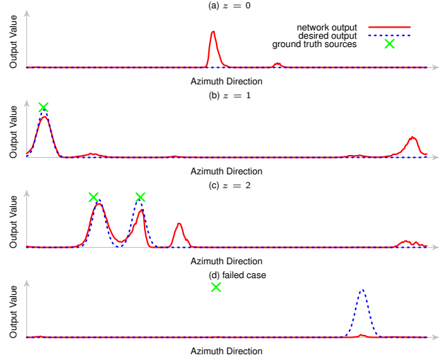
Fig. 3: Examples of output regularization with known number of sources. The desired output is the closest output in the reduced space to the actual network output. The ground truth locations are presented but not used for weak supervision.
