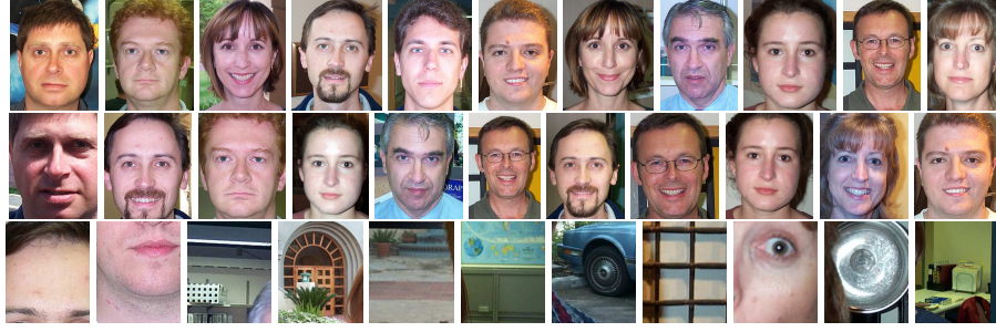
Fig.3. Bootstrapped images. Some initial positive images are shown at top row. After one bootstrapping iteration, the algorithm extracts new positive and negative samples. New positive images contain the target object at different scales and shifts (middle row). Contrary, new negative images contain difficult backgrounds and some portion of the object (bottom row).
