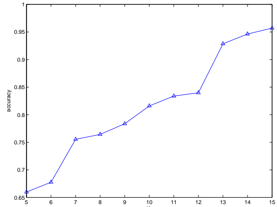
Figure 9: Classification performance of the algorithm for different values of parameter \mathcal{N} , i.e., the number of representatives each group g_m is represented by.
