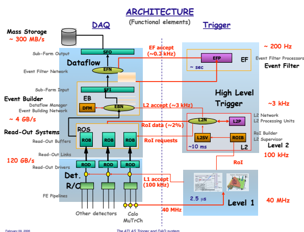
Figure 1: The ATLAS Trigger DAQ architecture.
