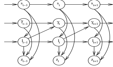
Figure 1: SIS Algorithm.
