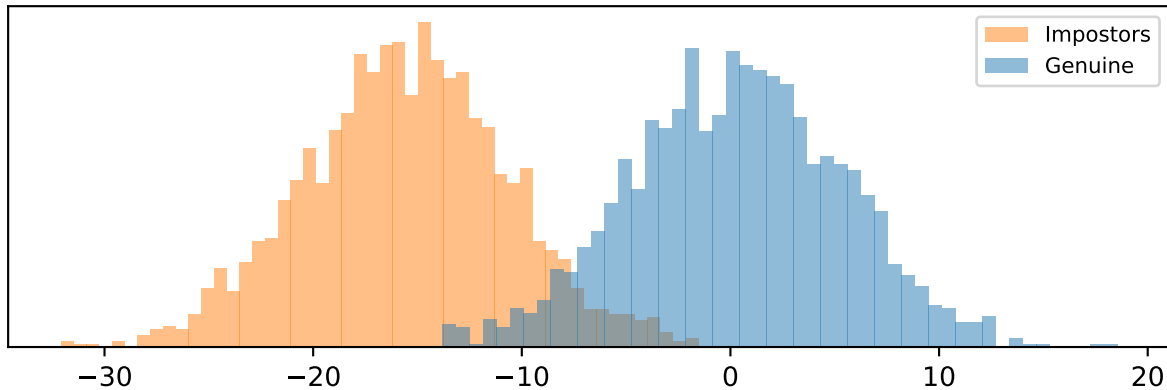
Z-norm scores
