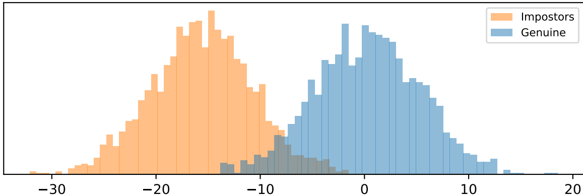
T-norm scores
