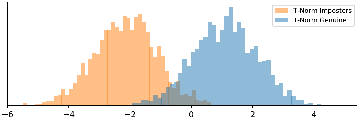
T-norm scores
