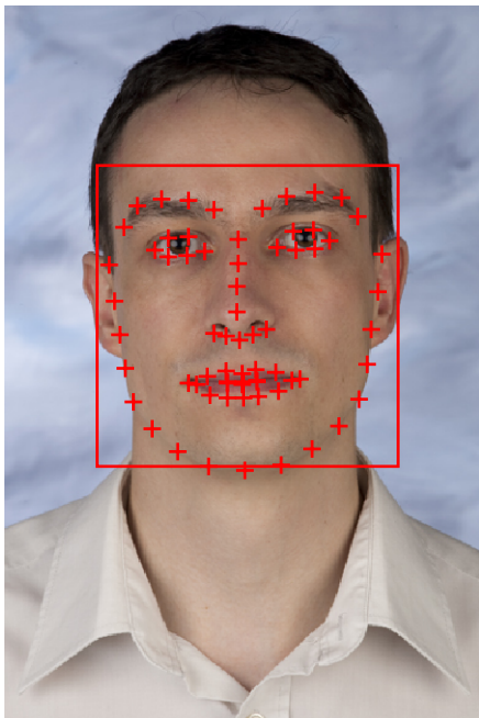
Dlib landmarks
