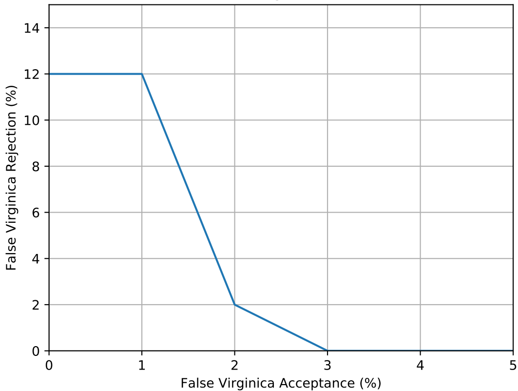
ROC Curve for Virginica Classification
