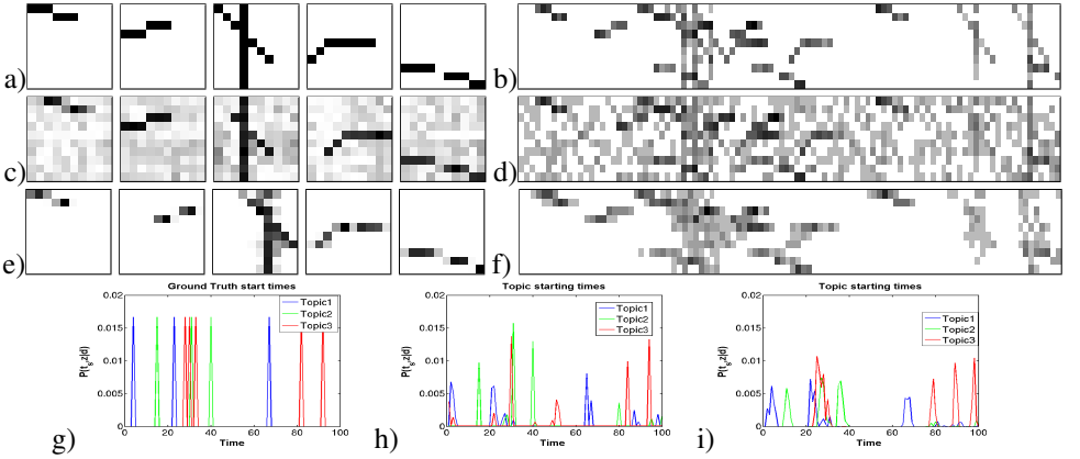
Figure 3: Synthetic experiments. (a,b,g) Clean data: (a) the five topics, (b) a segment of the generated document, (g) the topic occurrences (only 3 of them are shown for clarity). (c,d,h) experiments with uniform noise (the signal to noise ratio N_w^{\text{noise}}/N_w^{\text{true}} is 1): (c) the learnt topics, (d) the same segment as in (b) perturbed with noise, (h) the recovered topic occurrences p(z_t|d) . (e,f,i) (e) the learnt topics, (f) the noisy segment, and (i) the recovered topic occurrences, when adding a gaussian noise ( \sigma^2 = 1 ) on each word time occurrence t_a .
