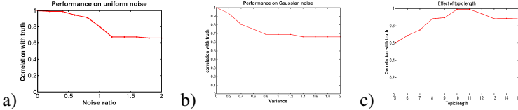
Figure 4: Average topic correlation between the estimated and the ground truth topics for different levels of (a) the uniform noise, (b) the Gaussian noise on a word time occurrence t_a , (c) Effect of varying topic length T_z from 5 to 15.
