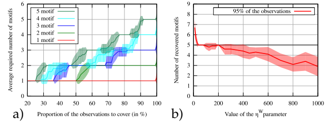
Fig. 27. Number of recovered motifs sufficient to explain a given proportion pr of the observations. Standard deviation is represented using shaded area. a) estimated number of motifs in function of the proportion pr , for different number (1 to 5) of motifs in the dataset. Note that when the threshold pr = 95\% , an accurate estimate of the number of motifs is found by our model. b) estimated number of motifs for different values of the weight \eta^W of the motif prior, and for 5 motifs in the ground truth.
