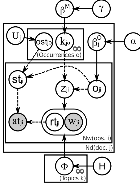
Figure 1. Proposed model using the stick-breaking convention. Dashed arrows represents deterministic relations (conditional distributions are a Dirac).
